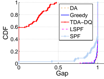
Fig. 8: Optimality gap
