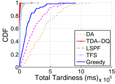
Fig. 7: Total tardiness
